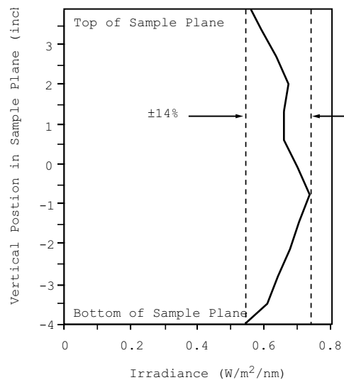
Figure 12 - Vertical Profile of Typical G53 Chamber
